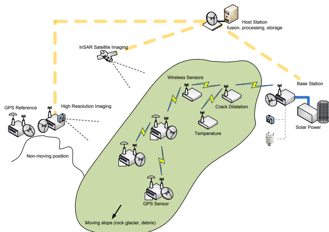
Figure 2. A multitude of sensor types as well as the fusion of information from different time and space scales are used for the detailed analysis of rock glacier terrain movement in the Swiss Alps.
