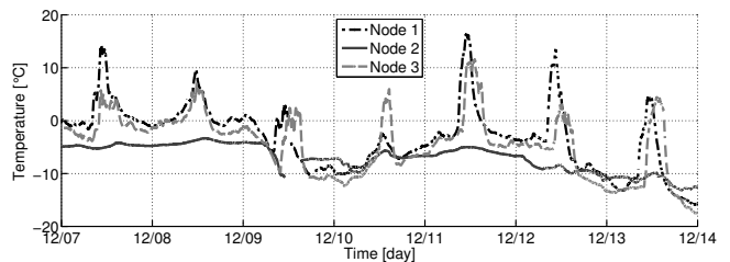
Figure 3. Temporal and spatial temperature variations.
