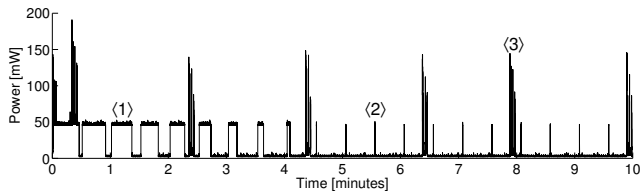
Figure 5. Disconnected operation of an isolated node.
