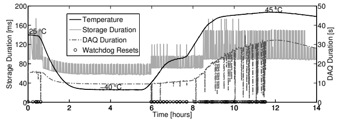
Figure 4. Effects of temperature variations on the duration of operations.
