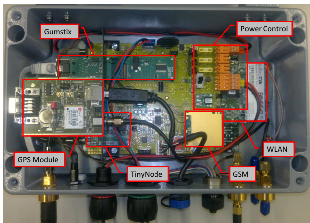
Figure 8. CoreStation : The motherboard provides extensive power control, system monitoring, and interface circuitry (e.g., to a GPS module). Interfaces to several communication links (WiFi, GSM modem, TinyNode radio) allow remote observation and control.
