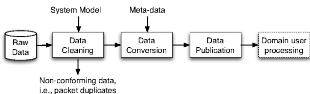
Figure 6. Collected raw data is firstly cleaned by involving a formal model of the data generation and transmission system. Conversion functions, calibration data and other meta-data are then used for converting raw readings to SI values.
